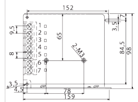
VOEDING 24Vdc - 200W max
