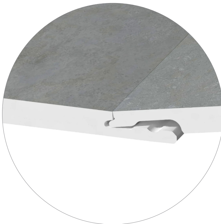
Detail click-systeem
