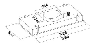
Slim motor (op unit) KACL.782#49F
