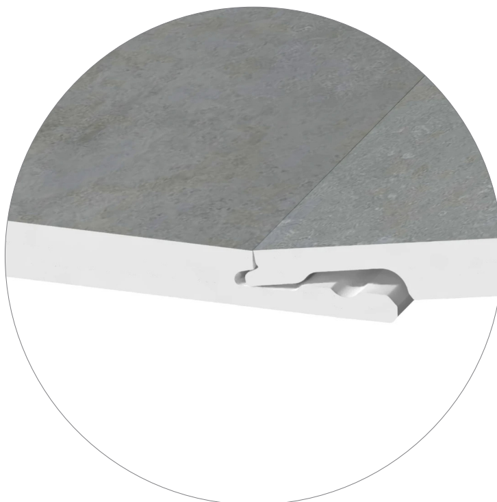
Detail click-systeem
